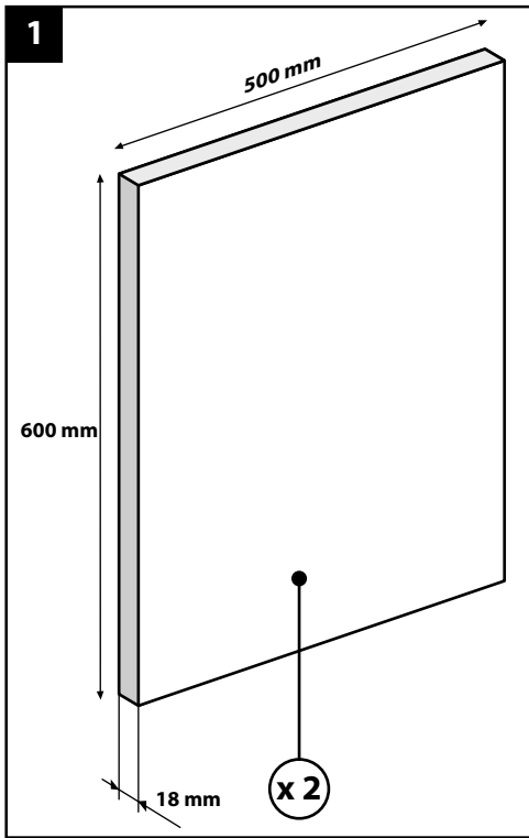
x 2 Planches bois 500 x 600 mm
